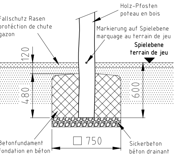
Fundament F03-R
