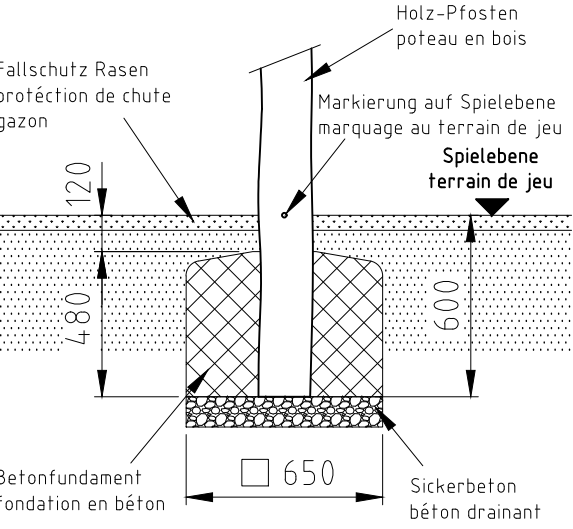
Fundament F03-R
