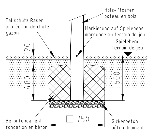
Fundament F03-R
