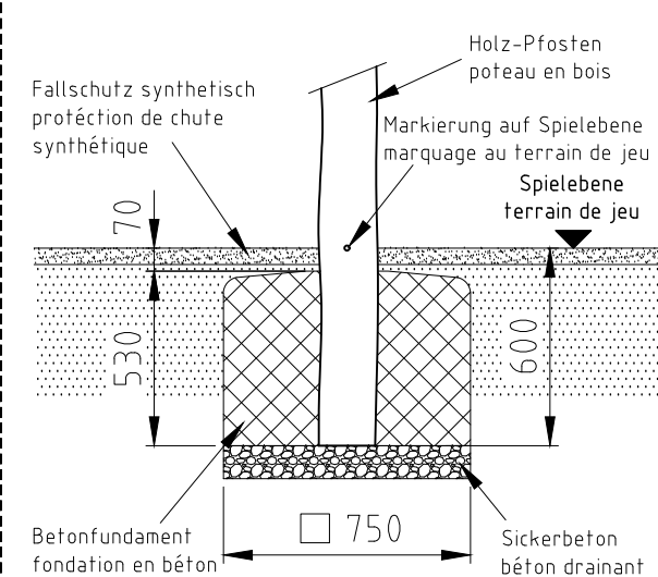
Fundament F03
