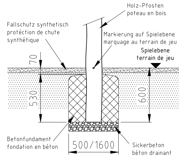
Fundament F02
