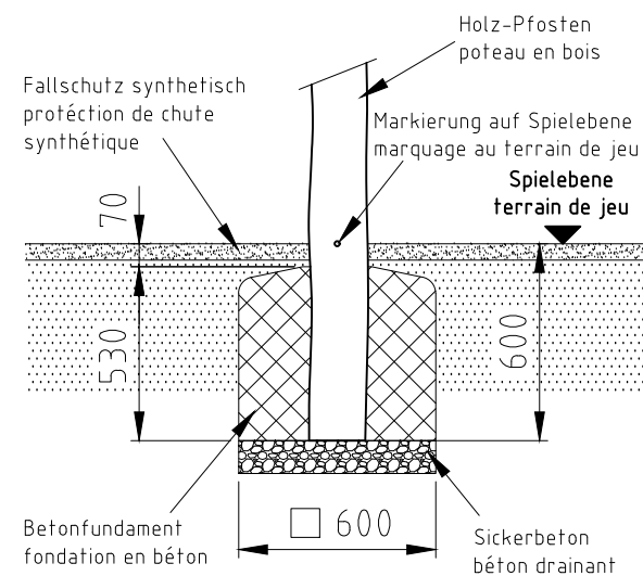
Fundament F02
