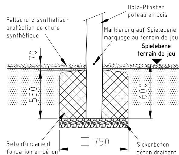
Fundament F03
