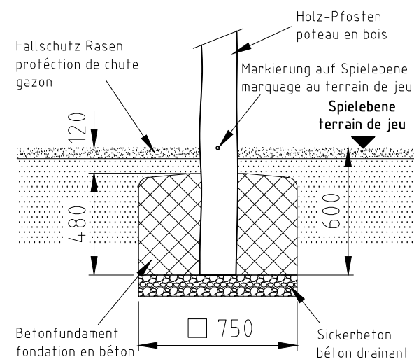
Fundament F03-R
