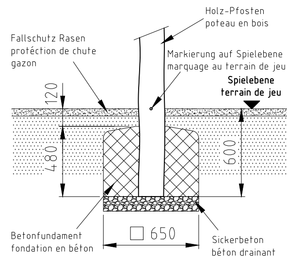
Fundament F02-R
