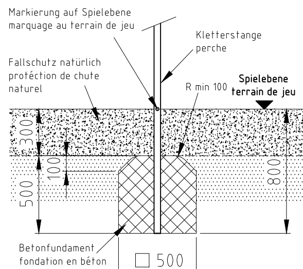
Fundament F05
