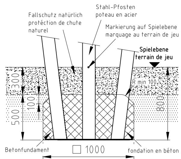
Fundament F05
