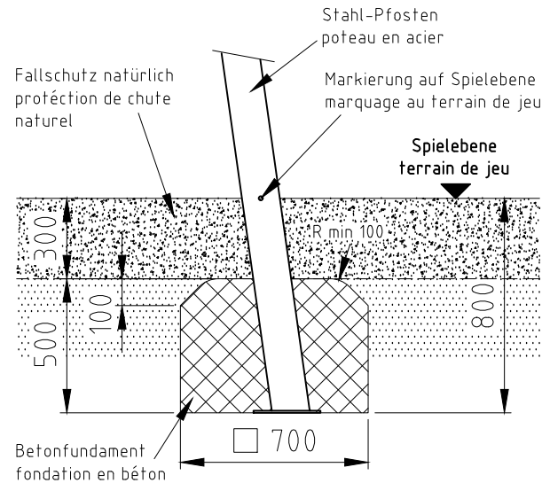
Fundament F09
