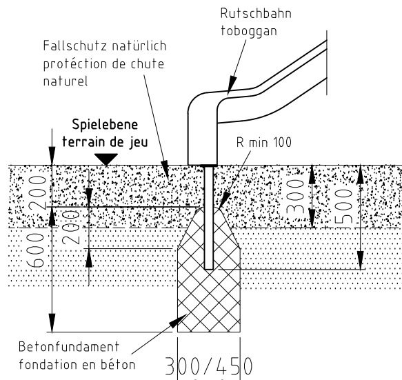
Fundament F09
