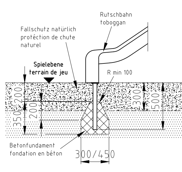
Fundament F09
