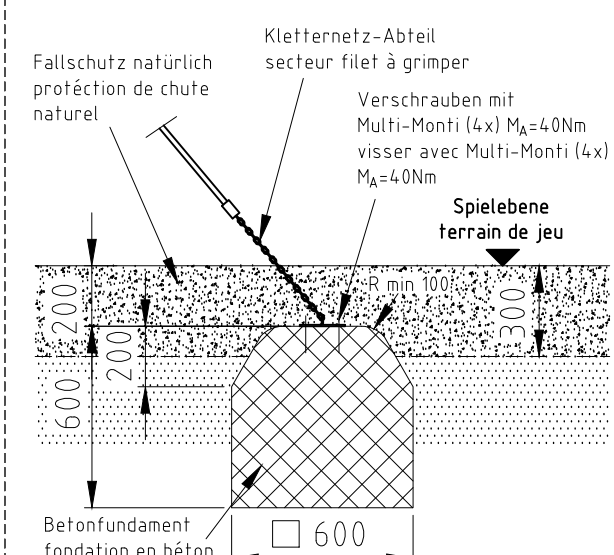
Fundament F08
