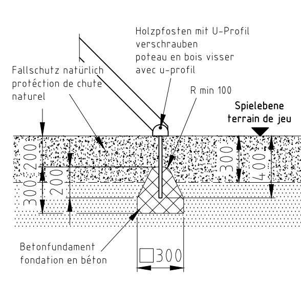
Fundament F03
